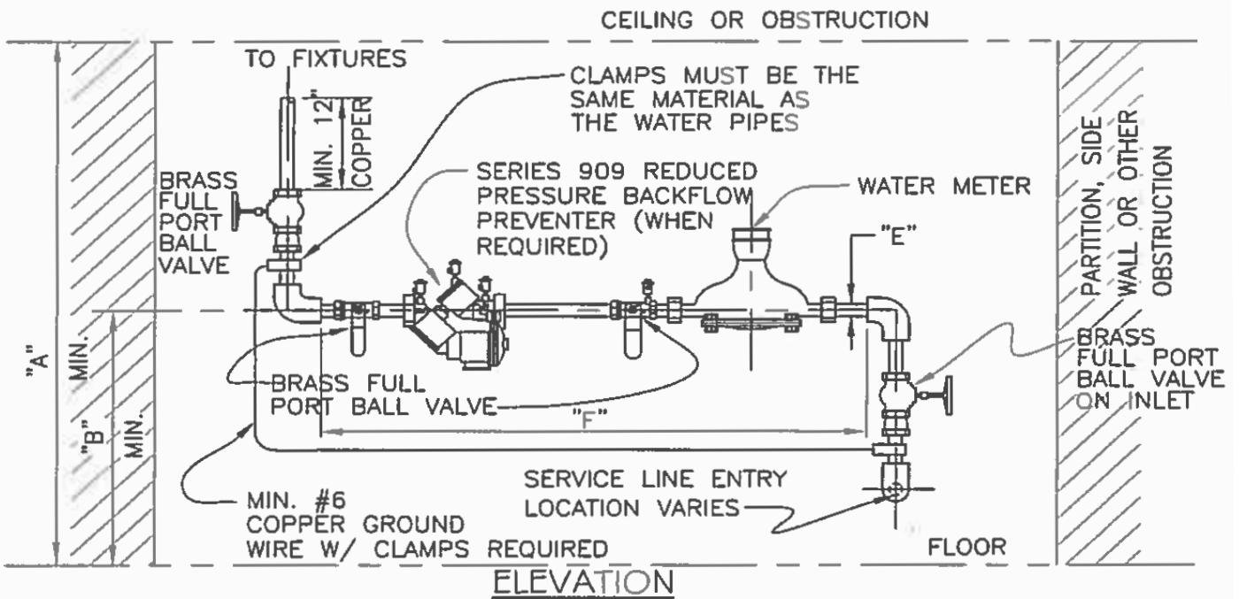
CLEARANCES FOR INDOOR WATER METER W/ BACKFLOW PREVENTION INSTALLATION
