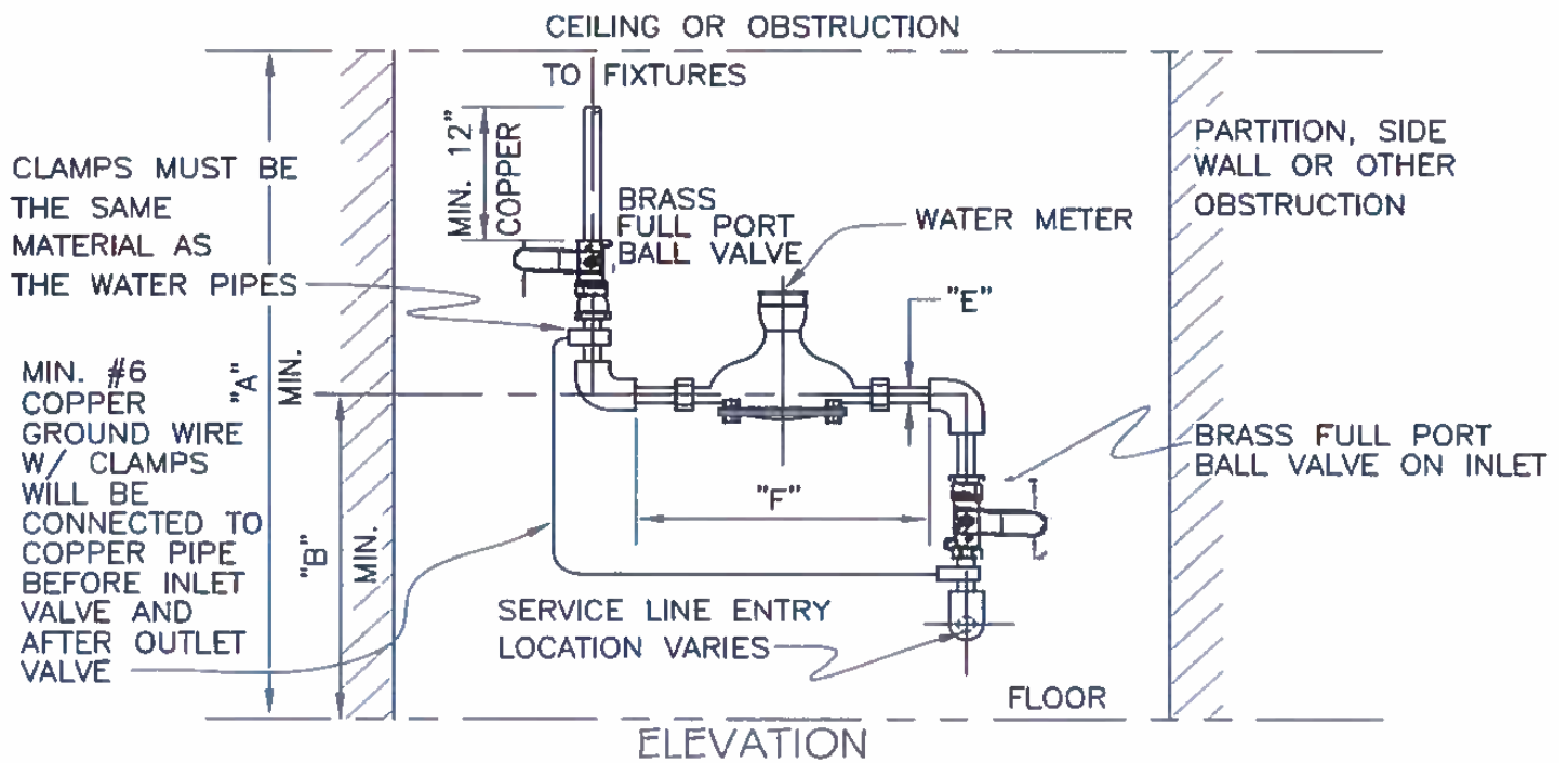
STANDARD CLEARANCES FOR INDOOR WATER METER INSTALLATION
