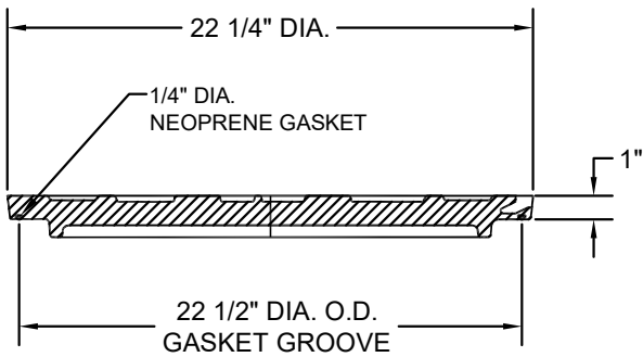
COVER SECTION
