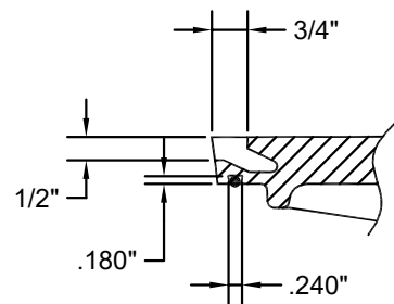
PICKHOLE DETAIL
