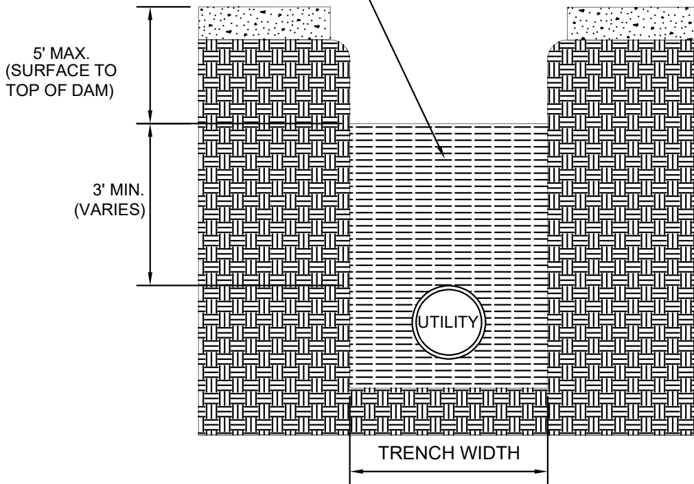
CROSS SECTION
