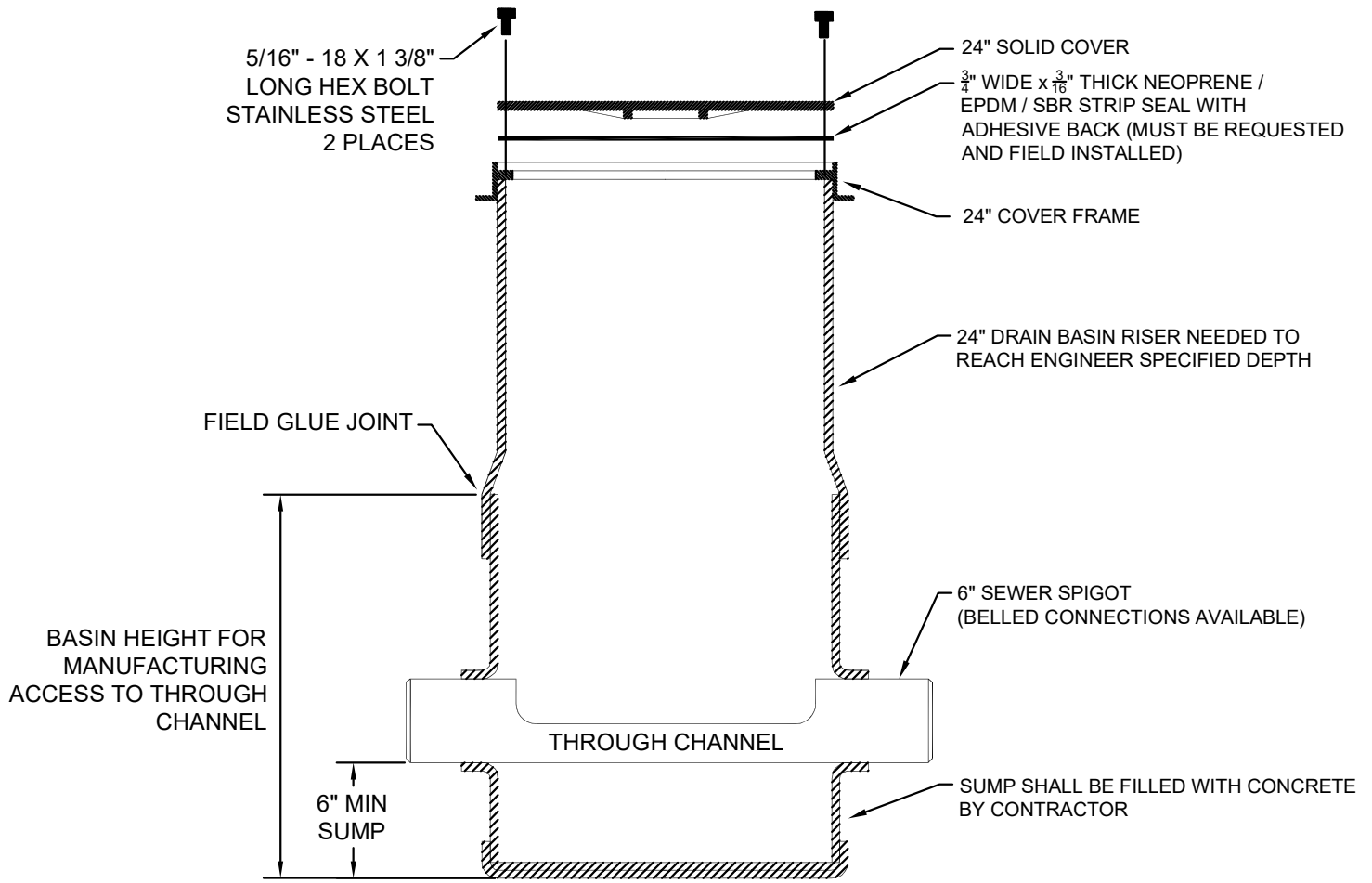
SECTION VIEW
