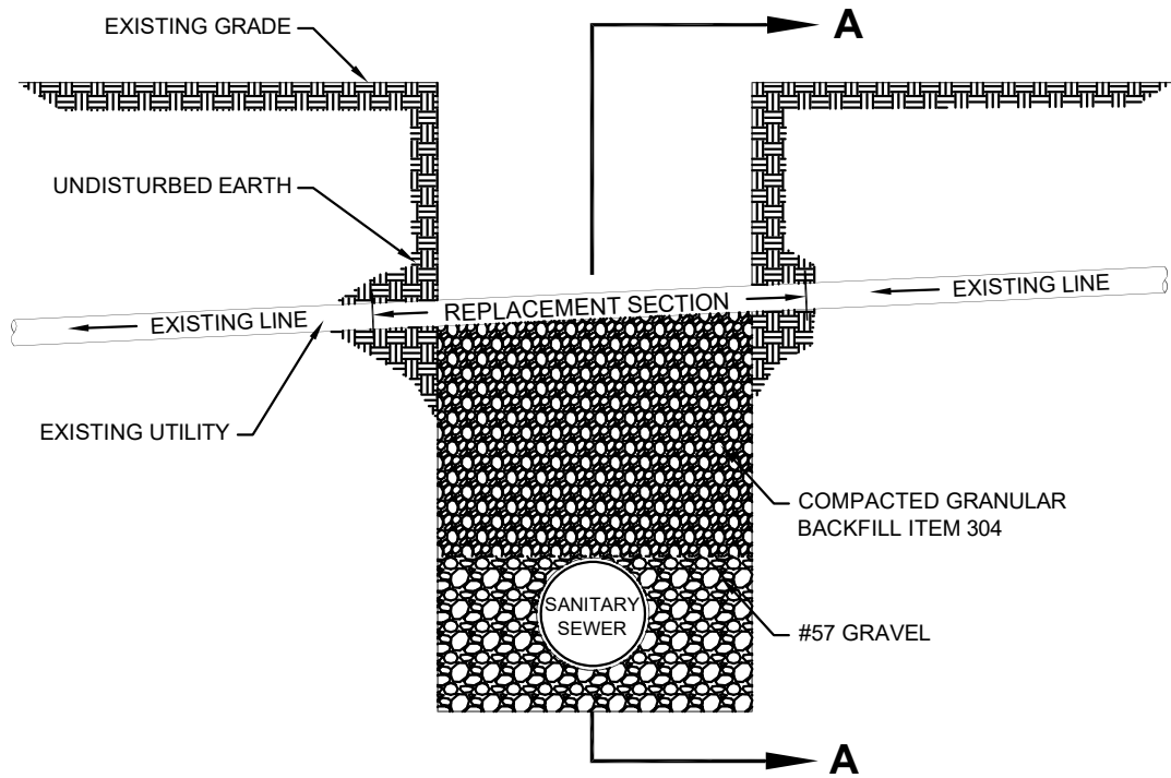
SECTION B-B
